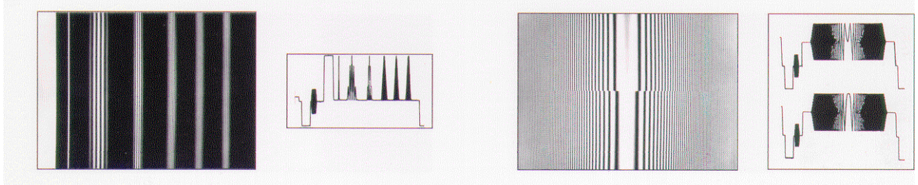
Examples of test signals (from left to right): multipulse, H sweep, sin x/x
